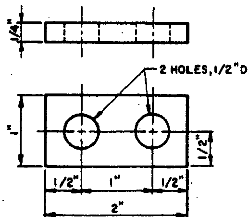
LOCK PIN Detail "B", 2-Req'd
