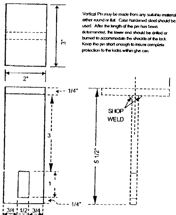
VERTICAL PIN Detail "C", 2-Reg'd
